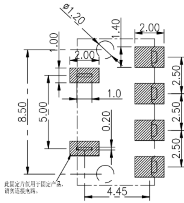
RECOMMENDED PCB LAYOUT TOP VIEW (.XX±0.05)
